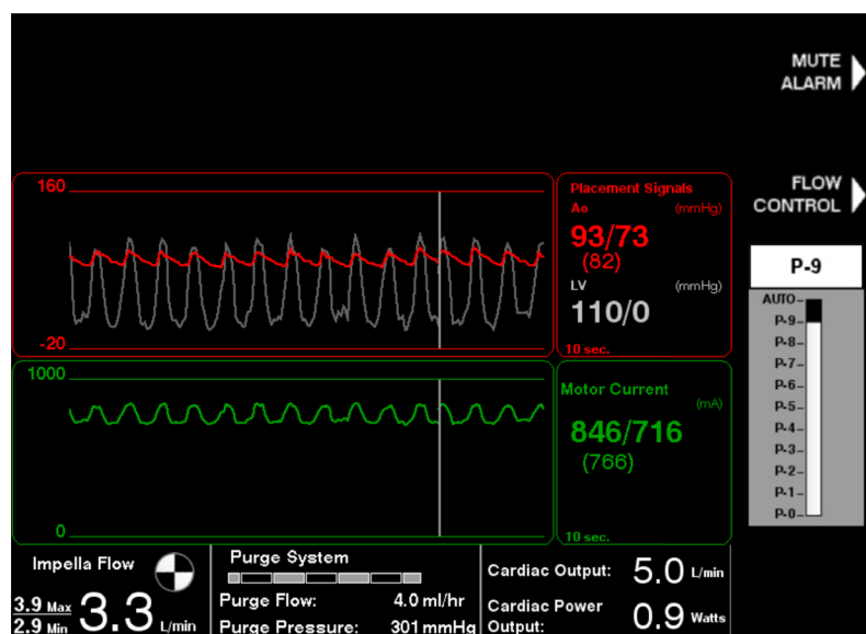
Figure 5.30 Adjusting P-level
