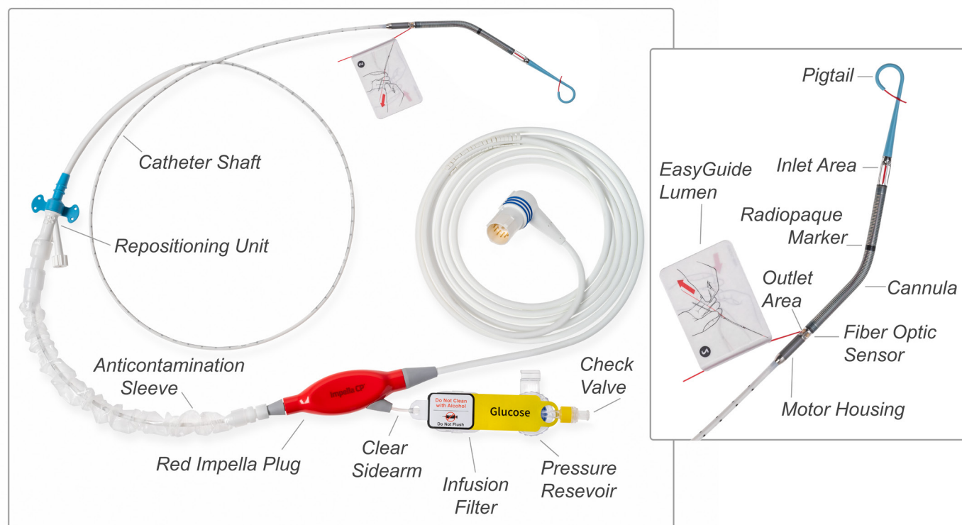
Figure 3.3 Impella Catheter
