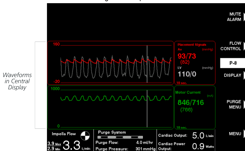
Figure 4.4 Placement Screen
