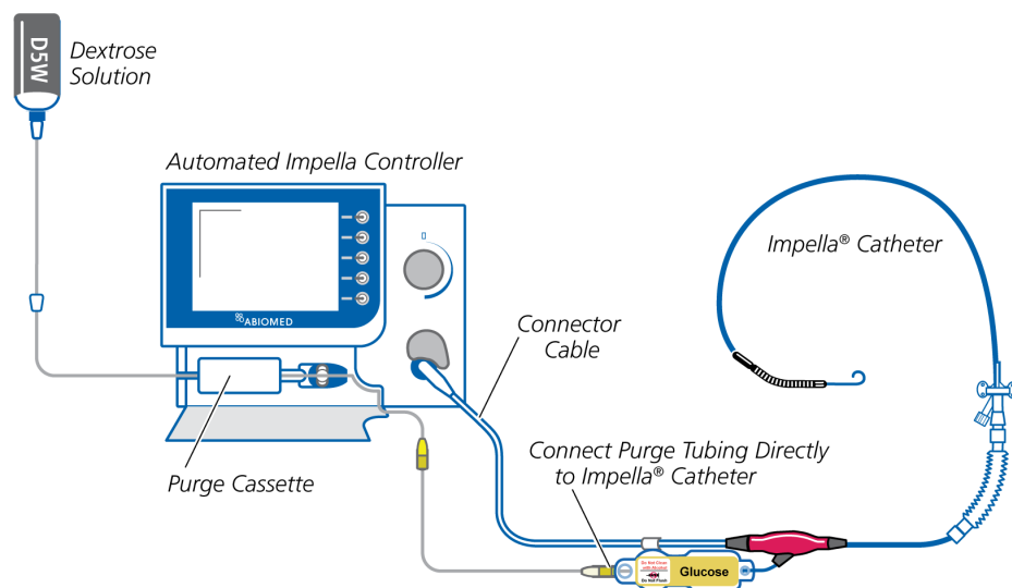
Figure 3.2 Set-up Configuration of the Automated Impella Controller, Impella CP with SmartAssist Catheter, and Accessories.
