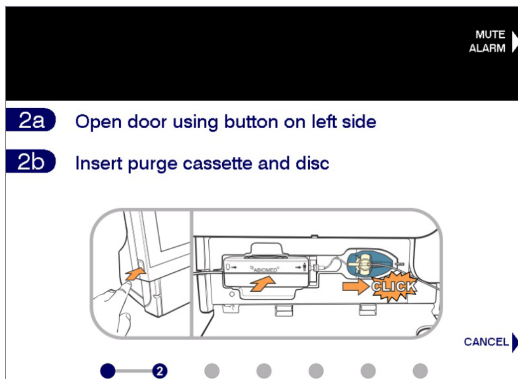
Figure 5.8 Inserting Purge Cassette into Automated Impella Controller
