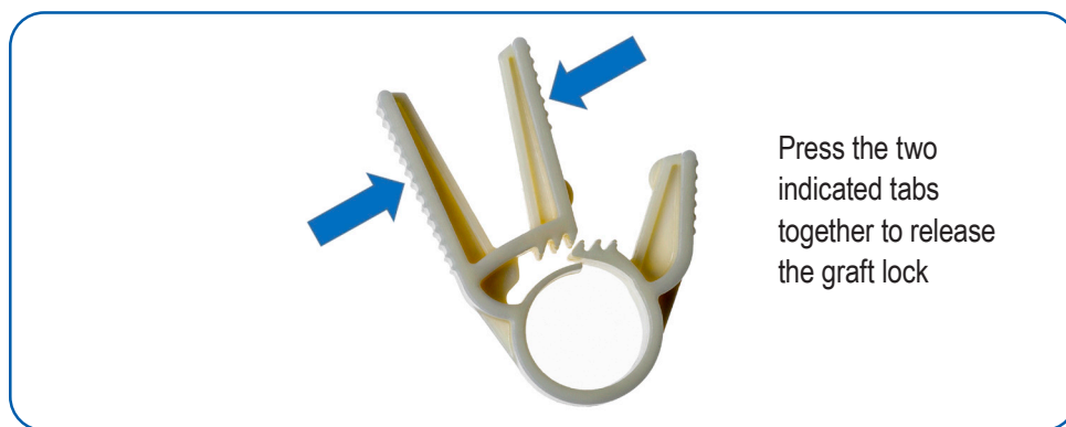
Figure 5.17 Releasing the Graft Lock
